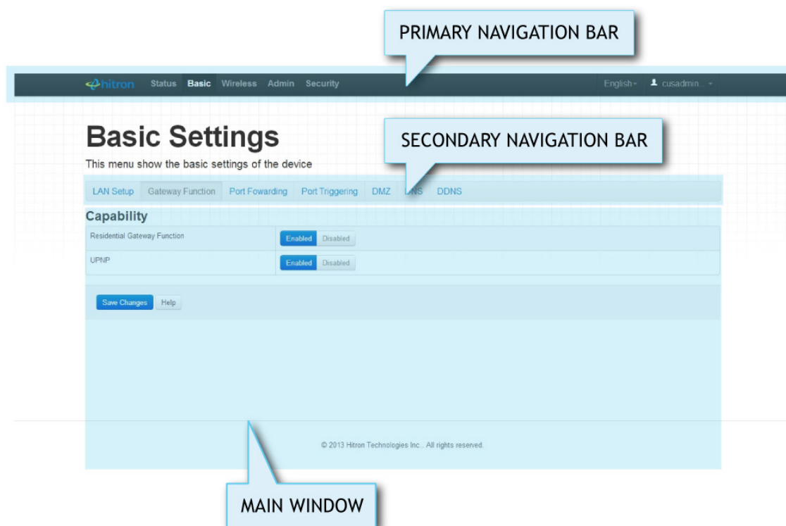
Figure 6: GUI Overview
