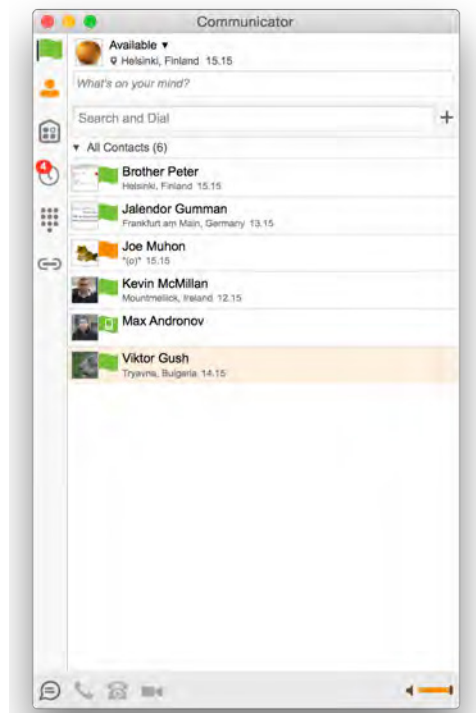
Figure 1 Main Window
