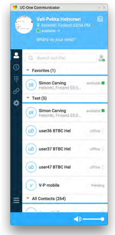
Figure 2 Chrome Application
