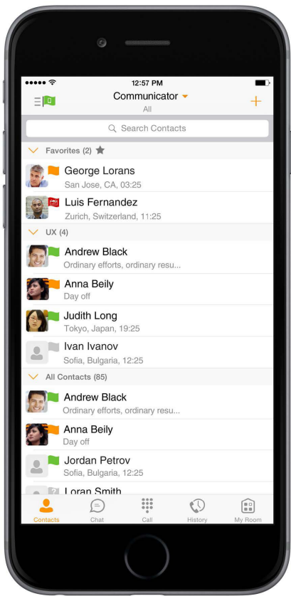
Figure 1 Main View
