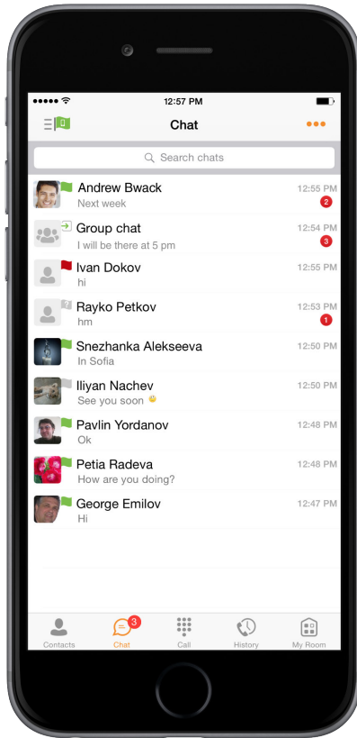
Figure 3 Chat Tab
