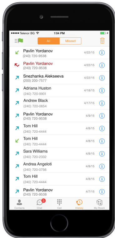
Figure 7 Call History
